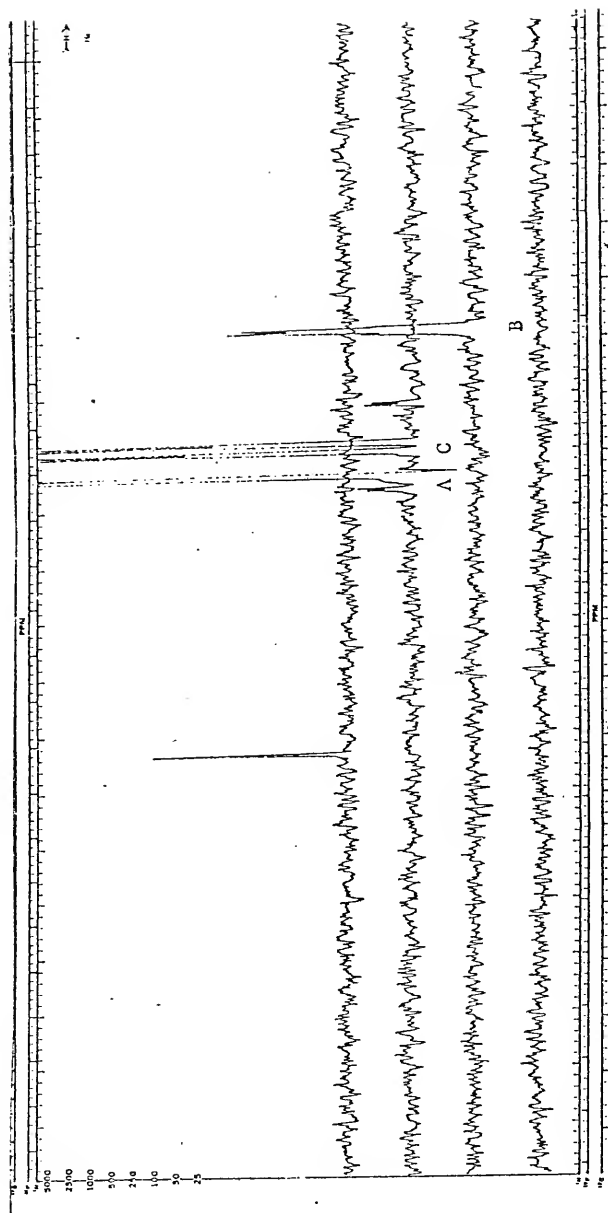
Figure 56 - ^{19}\text{F} NMR of \text{CF}_2\text{ClCFC1CH}=\text{CHCF}_3 A B C
